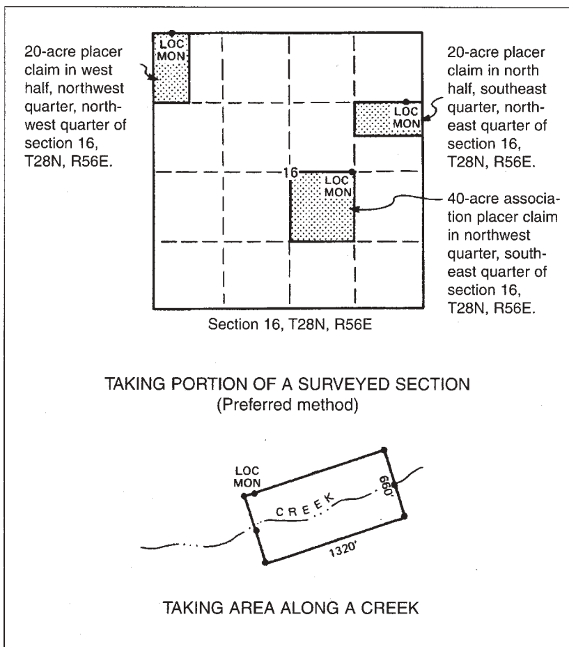
FIGURE 7. General form and monument locations for placer claims.
